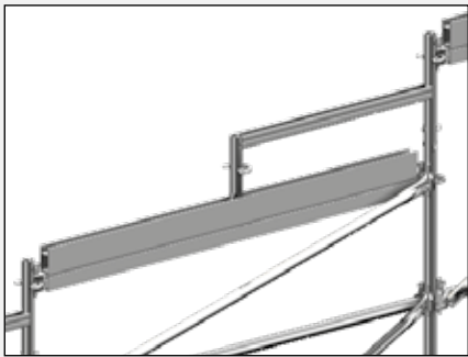
The stand element, 1-step 1 with a standard rise of 0.25 m is used for the Event systems EV 100 and EV 104.
