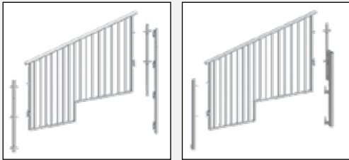
Variant for seating: Side guardrail in the system axis Variant for bench seat: Side guardrail next to the system axis
