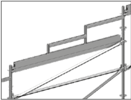
For the Event System EV 86, the stand elements, 2-step 2 with risers of 0.16 m, 0.25 m or 0.33 m are used.
